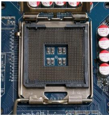
Intel Socket 775
