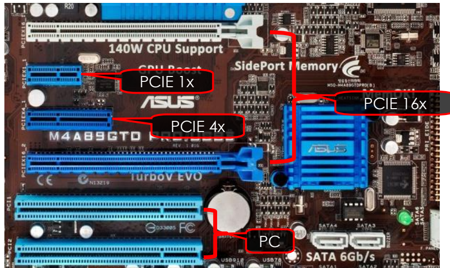
The expansion slots – PCI, PCI Express 1x, 4x and 16x
